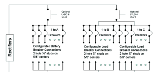
A+B = 20 + C for 19" shelves and A+B = 26 + C for 23" shelves. Each position in the primary panel is configurable for load or battery. All positions in the secondary panel are load.
