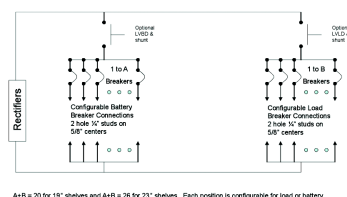
A+B = 20 for 19" shelves and A+B = 26 for 23" shelves. Each position is configurable for load or battery.
