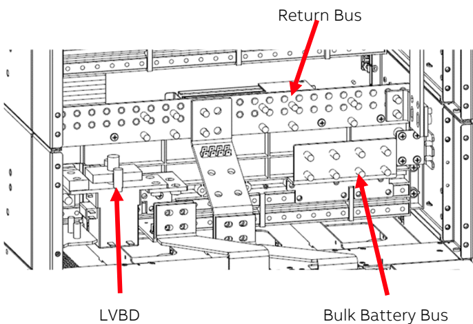
23" Dual Voltage System with 48V Primary & 12V Secondary Bus
