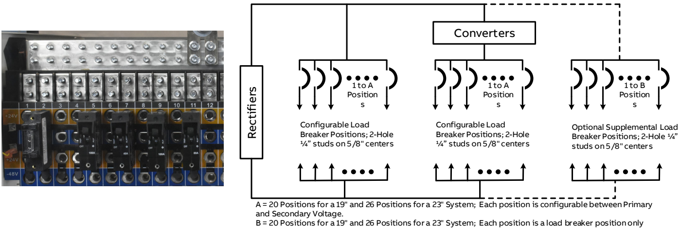
19" Dual Voltage system with Optional LVD
