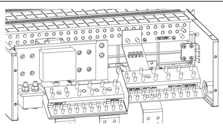
23" Dual Voltage system with Optional LVD
