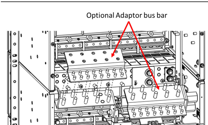
19" Dual Voltage system no LVD Option
