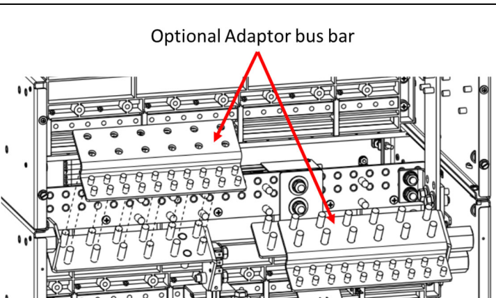
23" Dual Voltage system no LVD Option
