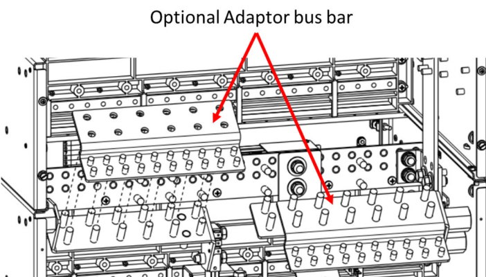
23" Dual Voltage system no LVD Option
