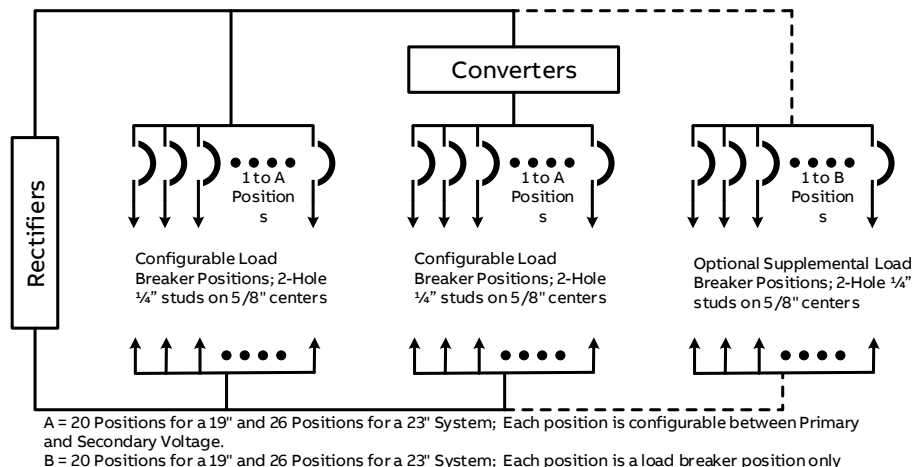
23" Dual Voltage system no LVD Option
