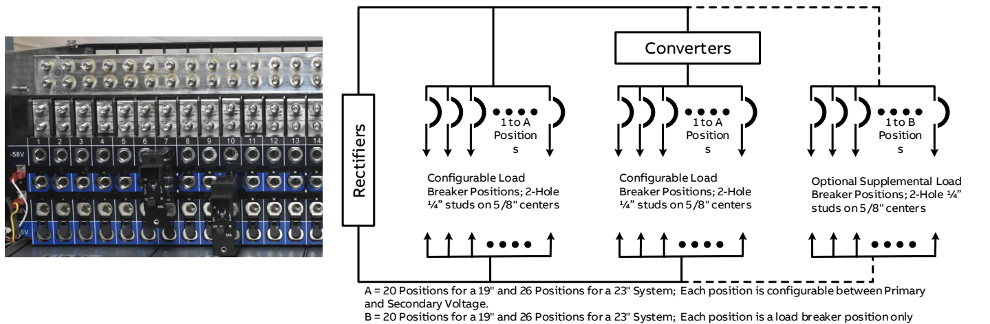
19" Dual Voltage system no LVD Option
