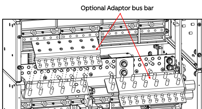
23" Single Voltage system without Battery Breaker bus
