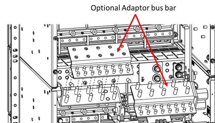
19" Dual Voltage system no LVD Option
