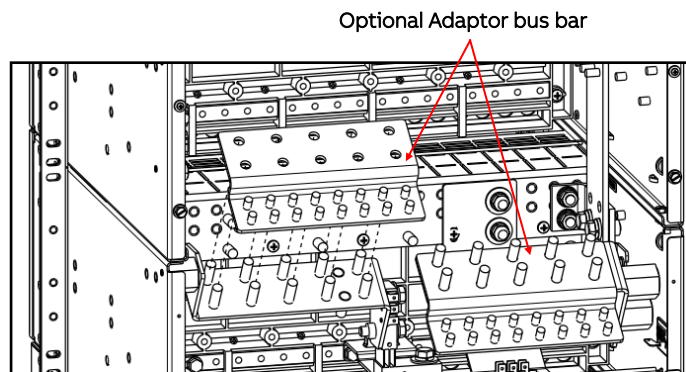
19" Single Voltage system without Battery Breaker Bus
