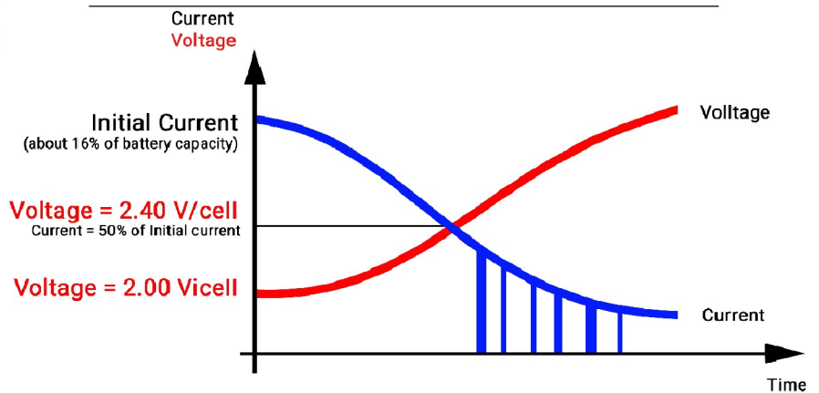
ETP Charging Profile "Wsa-Pulse"
